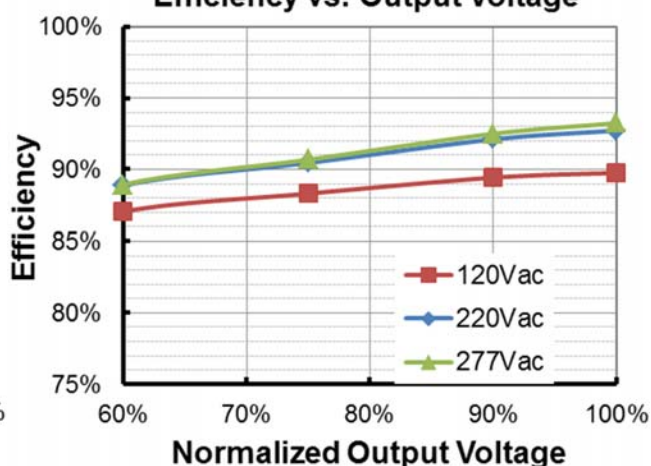
EUM-240S670Dx (Io=6700mA) Efficiency vs. Output Voltage
