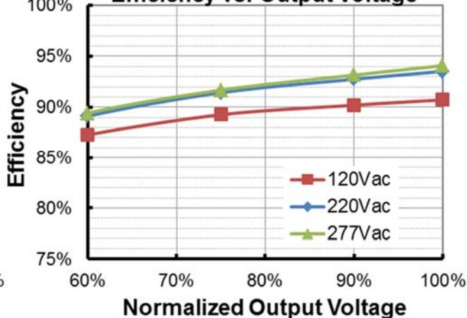
EUM-240S350Dx (Io=3500mA) Efficiency vs. Output Voltage
