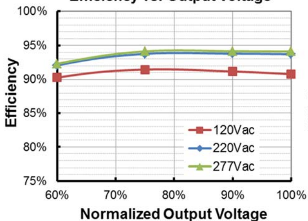
EUM-240S350Dx (Io=2150mA) Efficiency vs. Output Voltage
