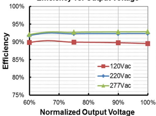
EUM-240S670Dx (Io=4200mA) Efficiency vs. Output Voltage
