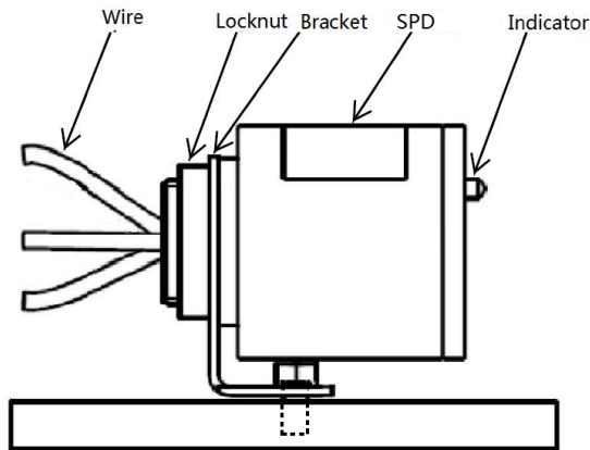
Bracket Installation
